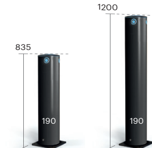
iFlex Cold Storage Bollard
